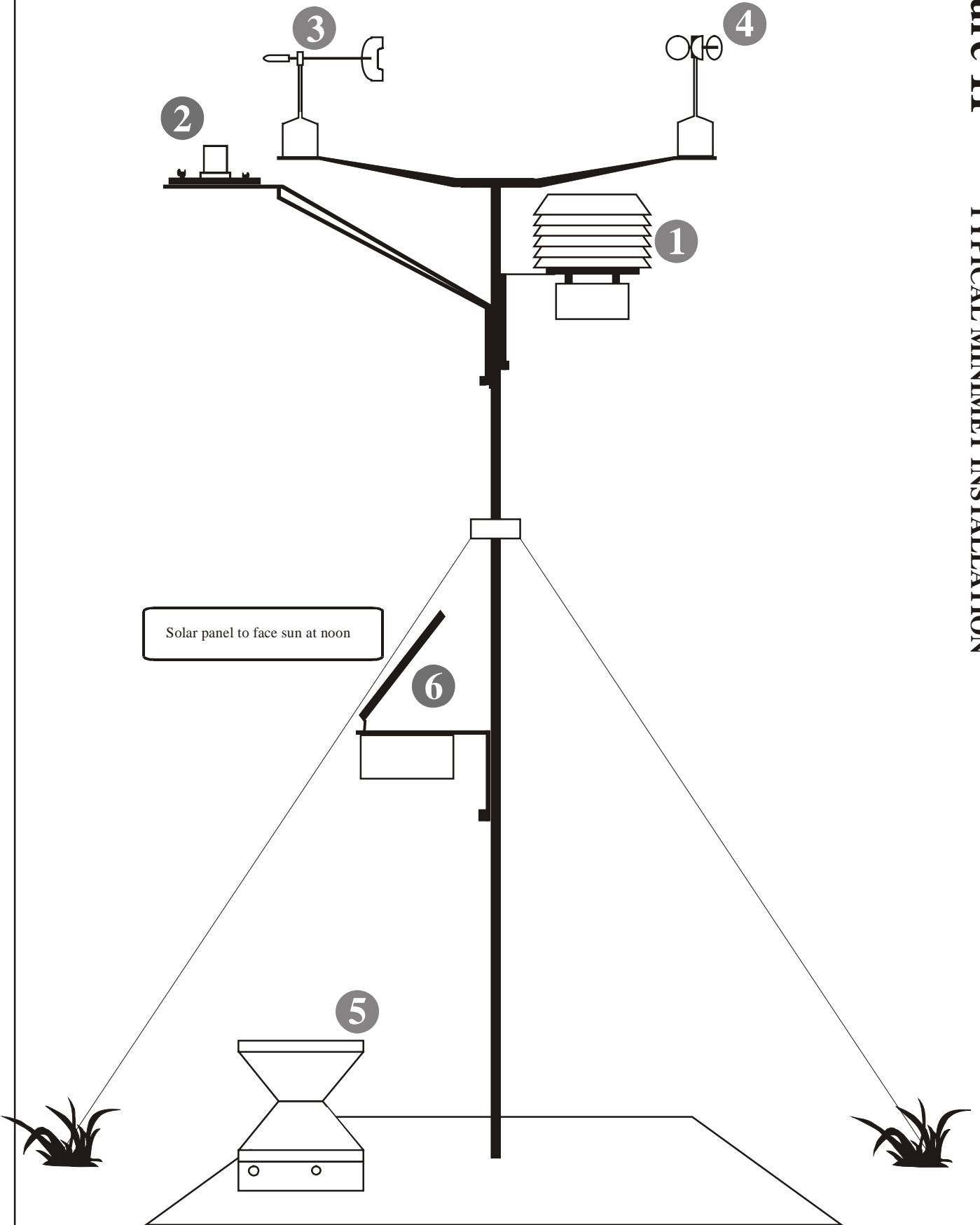
TYPICAL MINIMET INSTALLATION
